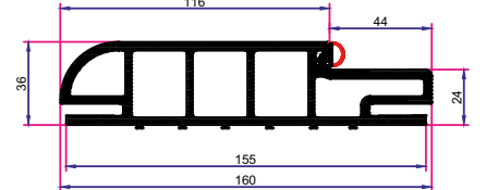
OVAL 160mm KAPI KASA
