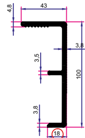
100x43x18 mm PERVAZ
