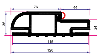
OVAL 120mm KAPI KASA
