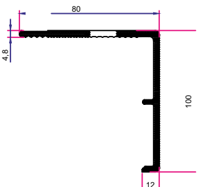
80x100 mm PERVAZ
