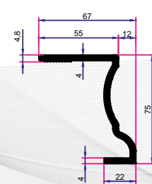
75x55 mm TA, PERVAZ
